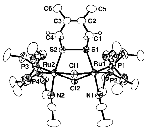
Figure 2. Structure of the cation 5 drawn at a 50% probability level. Methyl H atoms are omitted for clarity. Selected bond lengths [Å] and angles [°]: Ru1-S1 2.317(2), Ru2-S2 2.316(2), Ru1-P1 2.230(2), Ru1-P2 2.233(2), Ru2-P3 2.236(2), Ru2-P4 2.231(2), Ru1-Cl1 2.468(2), Ru1-Cl2 2.472(2), Ru2-Cl1 2.484(2), Ru2-Cl2 2.480(2), S1-S2 2.176(3), S1-C1 1.821(8), S2-C4 1.825(8), C1-C2 1.519(11), C2-C3 1.304(12), C3-C4 1.527(12), C2-C5 1.507(12), C3-C6 1.508(11); Ru1-S1-S2 108.12(10), Ru2-S2-S1 107.27(10), Ru1-S1-C1 114.4(3), Ru2-S2-C4 114.6(3), S1-C1-C2 110.3(6), S2-C4-C3 110.4(6), C1-C2-C3 117.6(8), C1-C2-C5 116.0(8), C5-C2-C3 126.4(9), C2-C3-C4 118.4(8), C4-C3-C6 116.3(8), C2-C3-C6 125.3(9).
